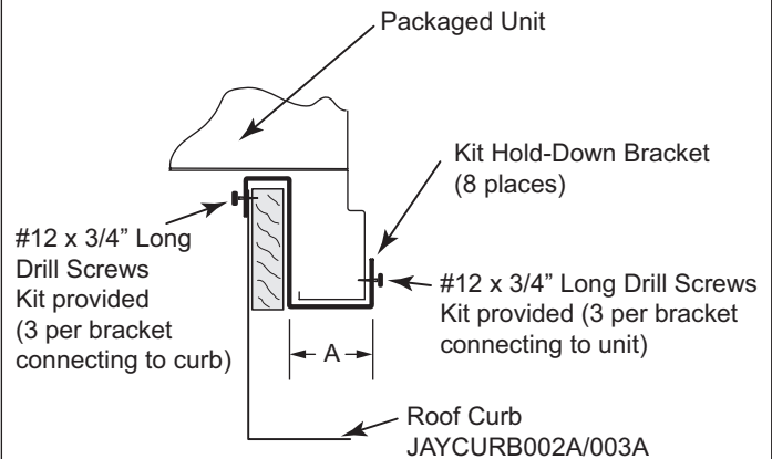
Figure 1. JAYEXMK002A/003A Installation Unit Mounted To Full Perimeter Curb
