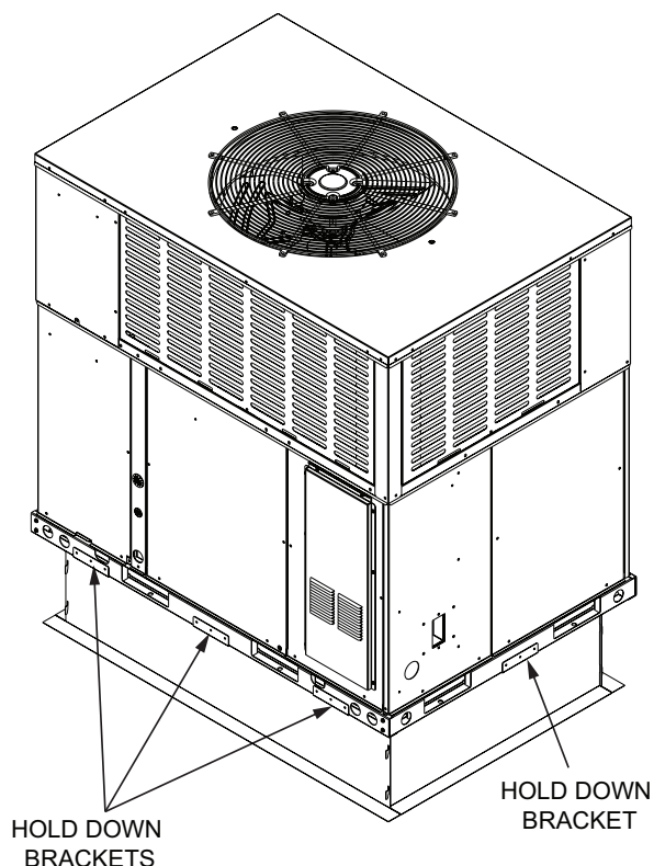
Figure 2. JAYEXMK002A Bracket Locations on *****24 – 42 Models
