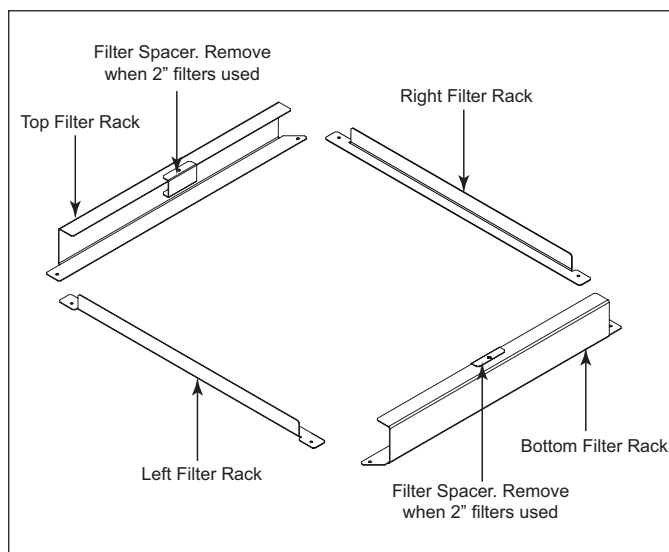
Figure 1. Filter Kit Components
