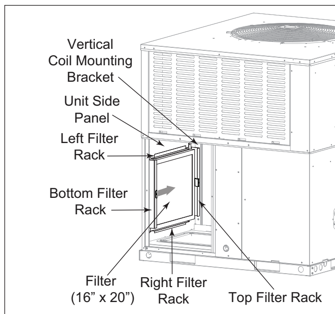
Figure 6. Horizontal Installation – Filter Rack Locations
