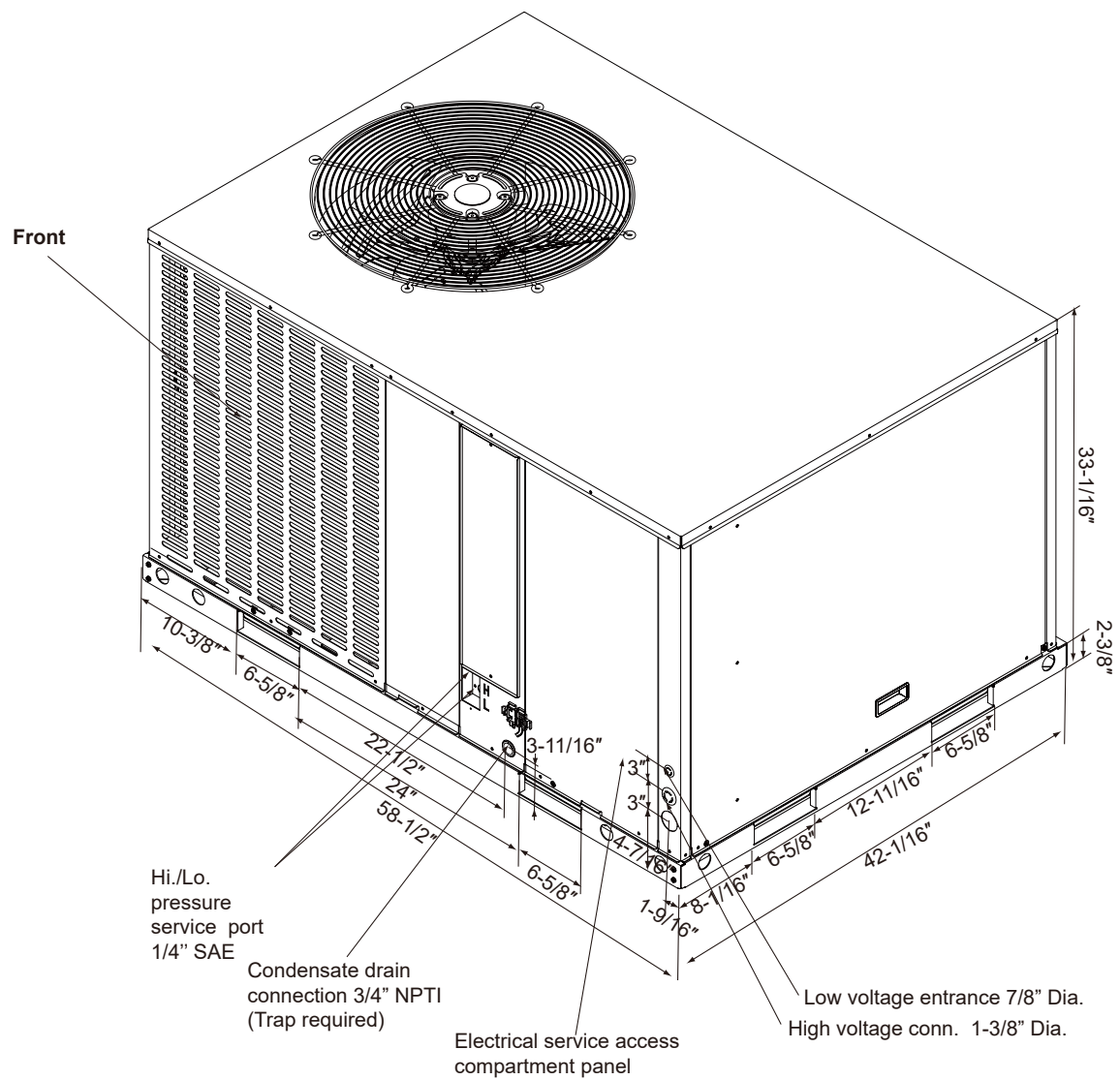
Fig. 2-4 Unit Dimensions
