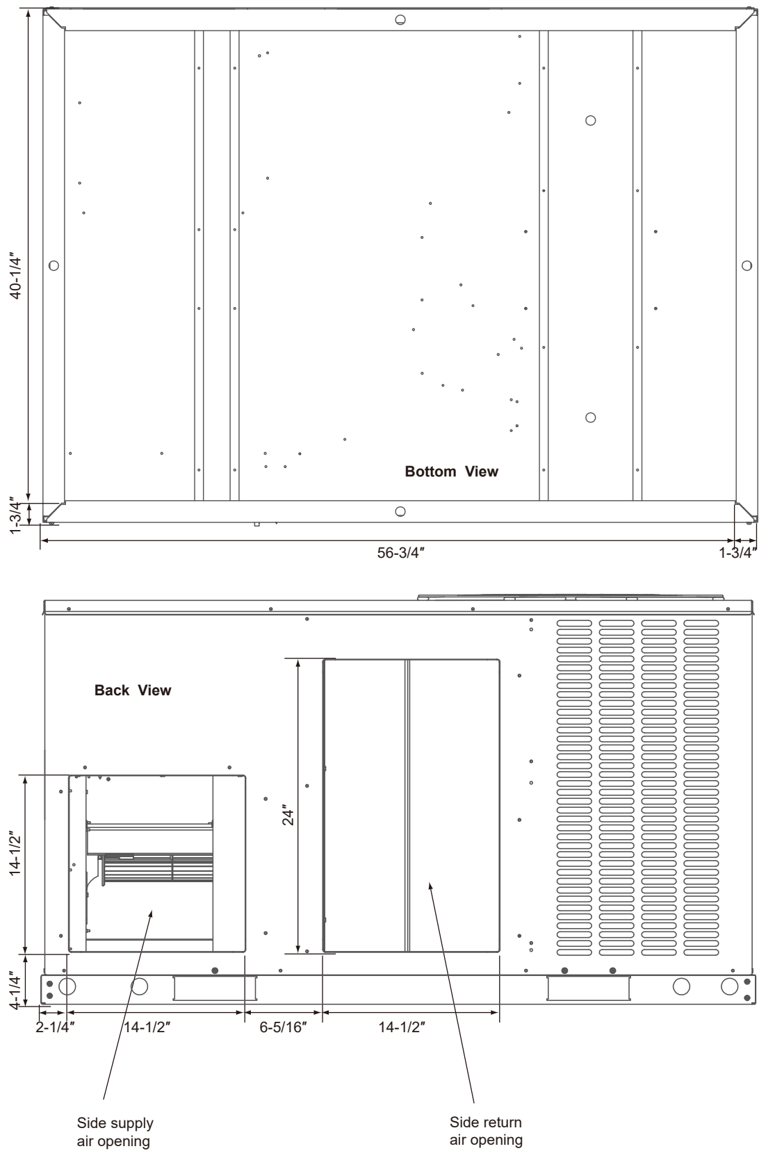
Fig. 2-5 Dimensions Back and Bottom
