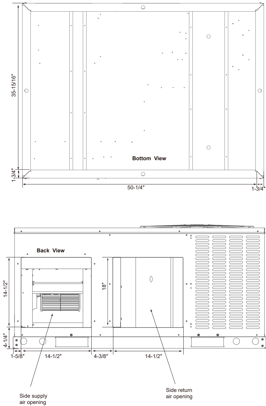
Fig. 2-3 Dimensions Back and Bottom
