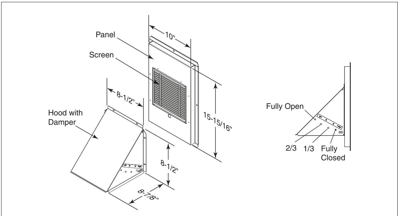
Figure 1. JAYOSAH002A Dimensions, Damper Settings
