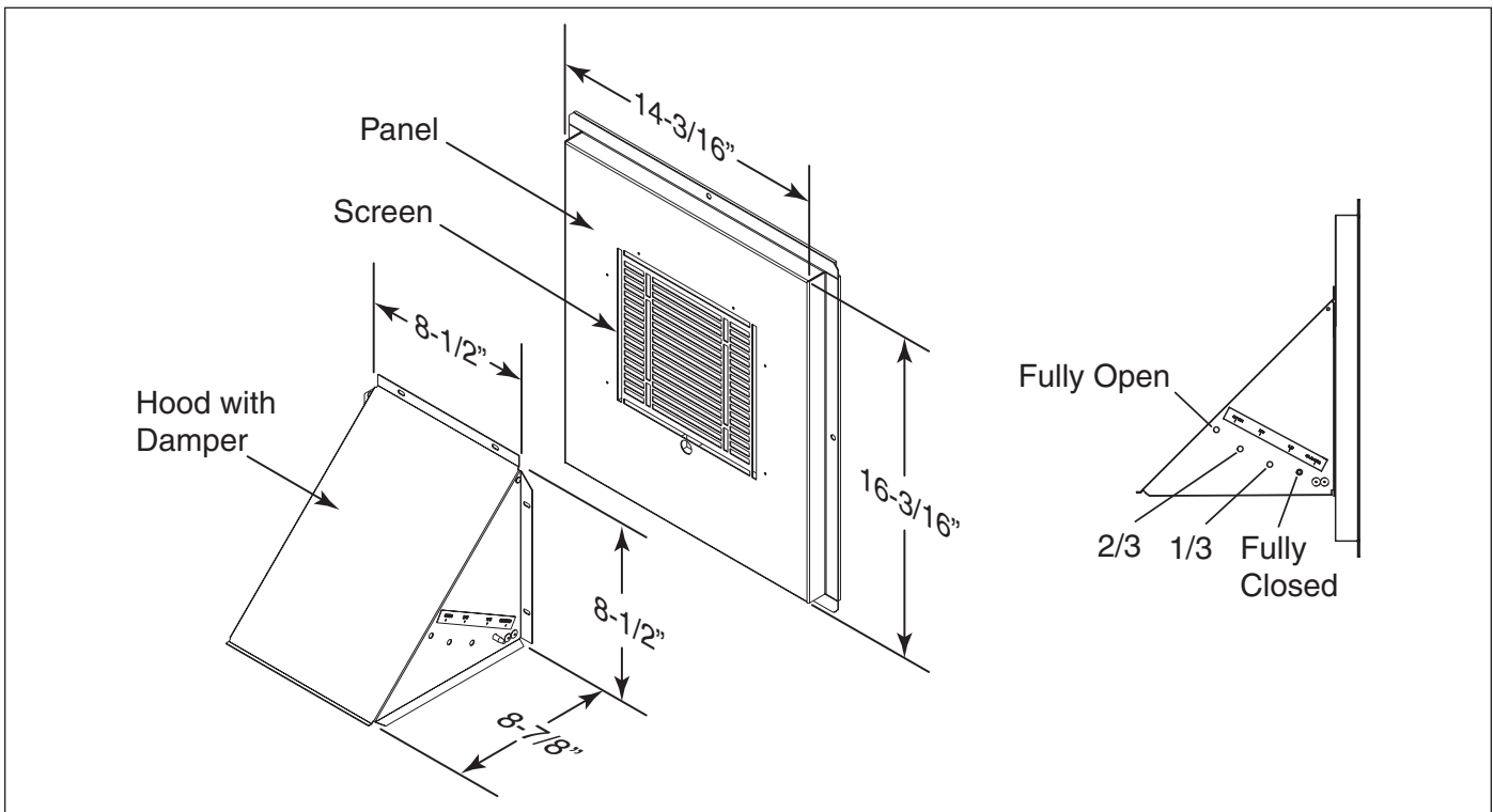
Figure 1. JAYOSAH003A Dimensions, Damper Settings
