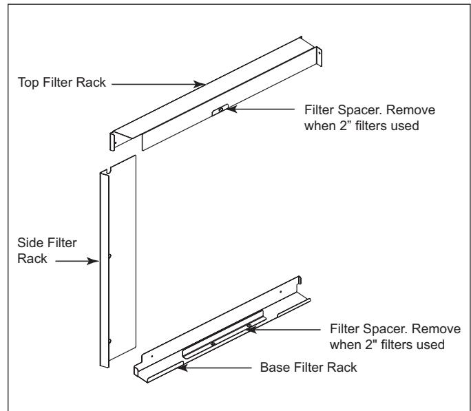
Figure 1. Filter Kit Components
